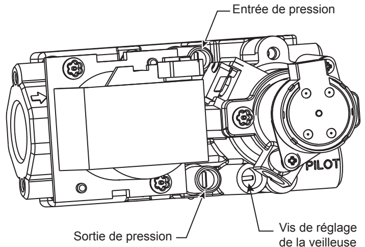
Figure 20 - Soupape de commande Signature
