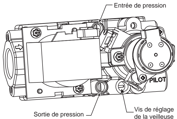
Figure 18 - Soupage de commande Signature
