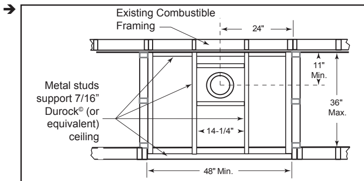
Figure 23 - Reflected ceiling plan.
