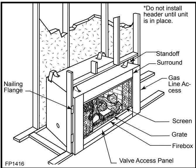
Fig. 8 Parts identification.
