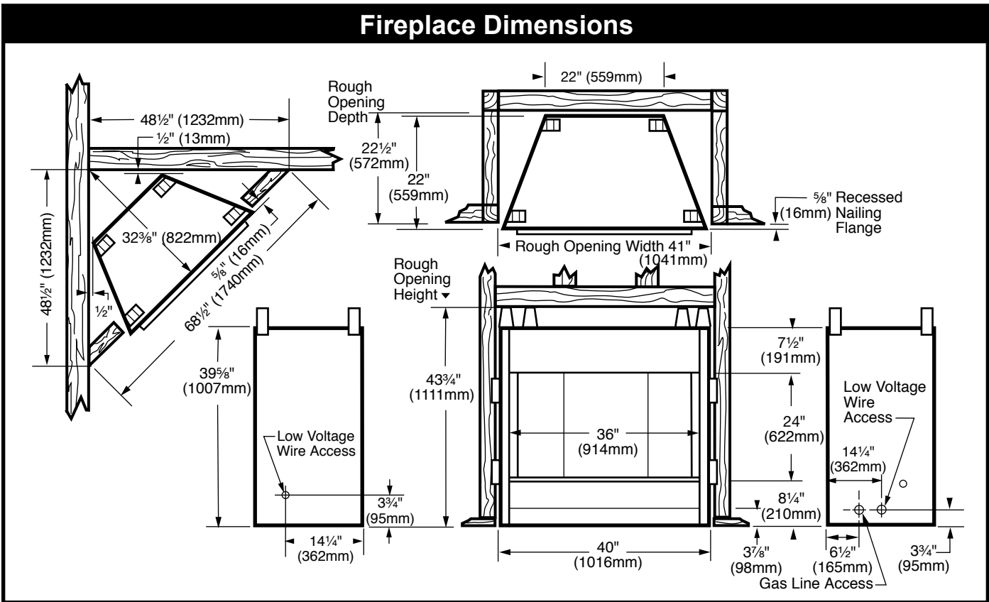
Fig. 1 ODGSR36A specification and framing dimensions.
