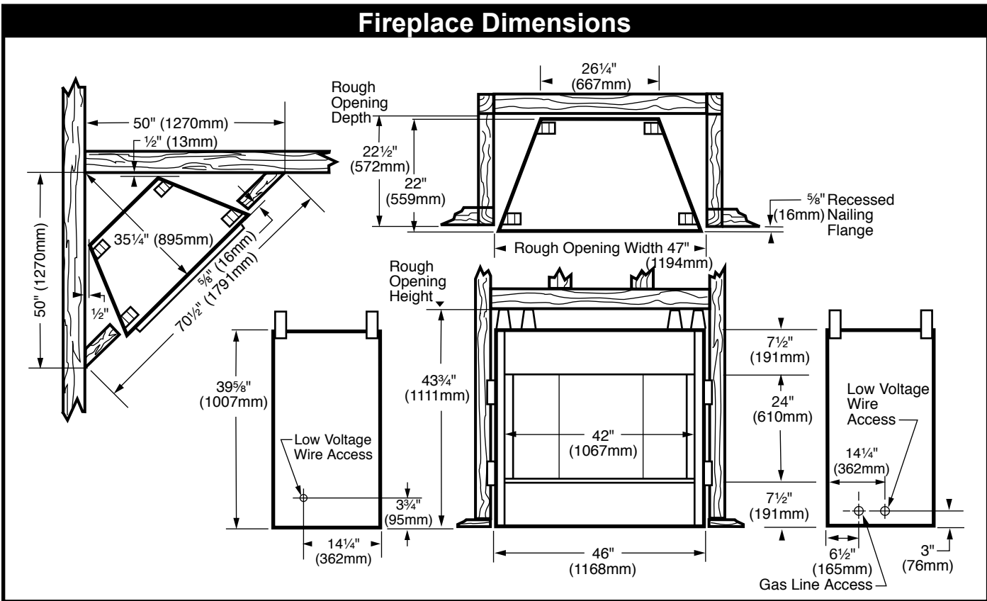
Fig. 2 ODGSR42A specification and framing dimensions.
