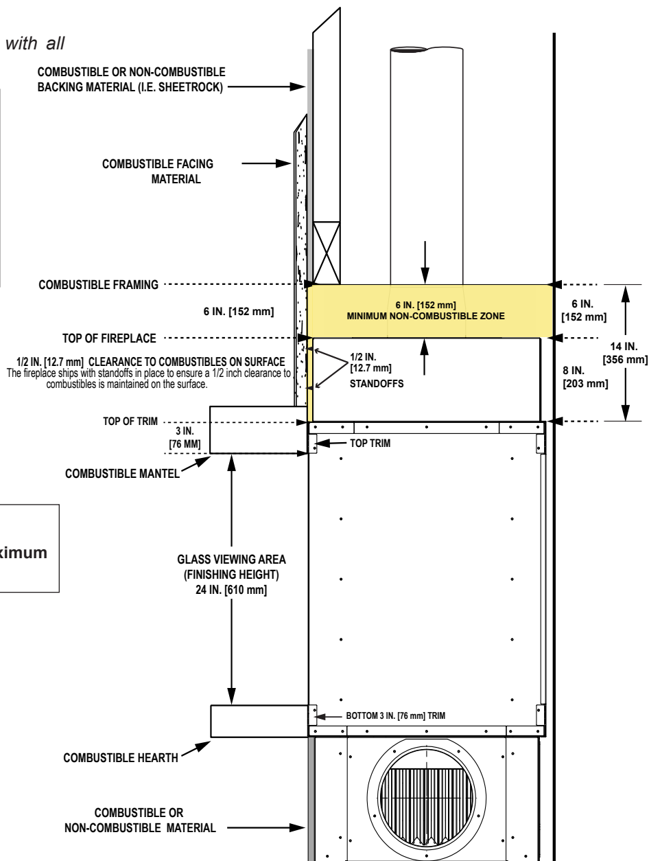
1/2" [12.7mm] Standoff
