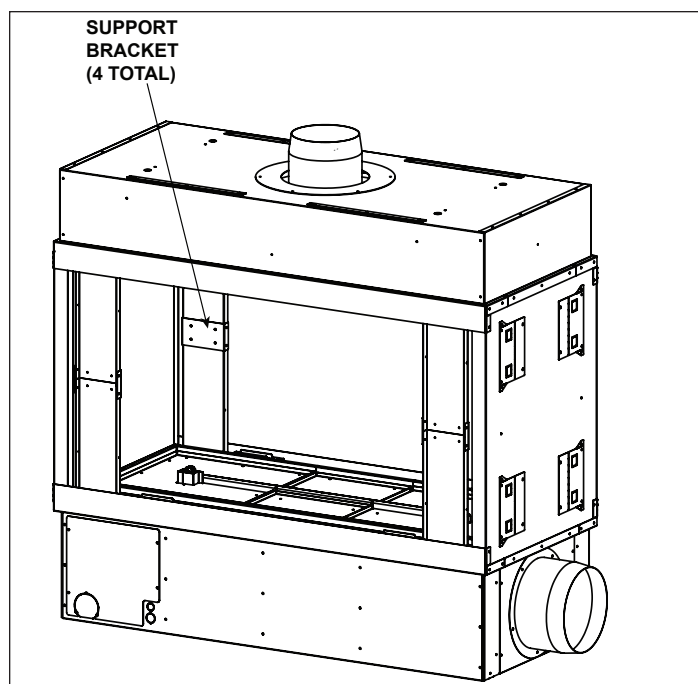
Figure 4.1 Temporary Shipping Support Bracket
