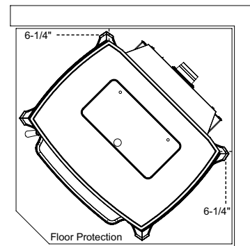
Corner Installation
