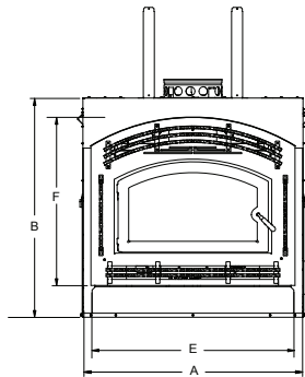
Arched Front View
